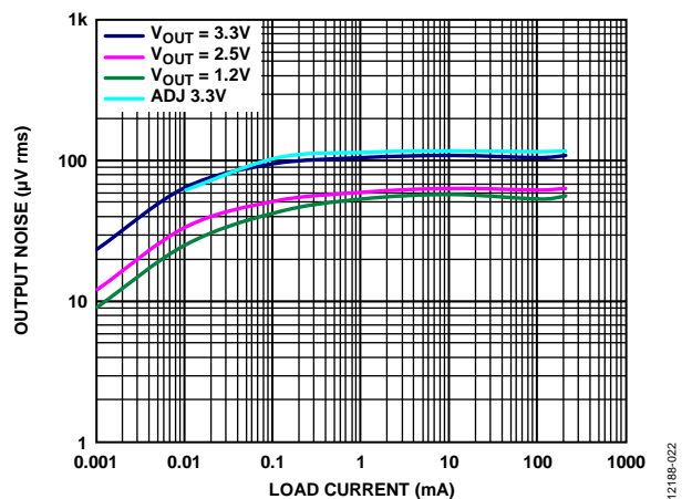
Figure 26. Output Noise vs. Load Current and Output Voltage, V_{IN} = 5\text{ V} , C_{OUT} = 1\text{ }\mu\text{F}
