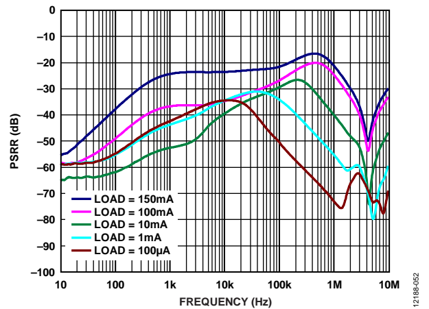
Figure 24. PSRR vs. Frequency, Various Load Currents, V_{OUT} = 3.3\text{ V} , V_{IN} = 3.8\text{ V}
