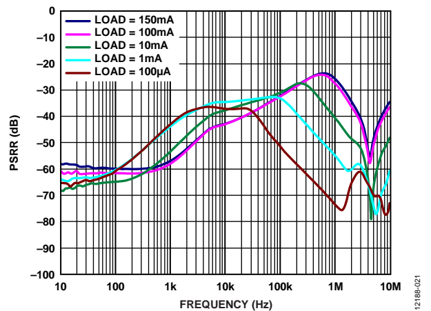
Figure 25. Adjustable ADP165/ADP166 PSRR vs. Frequency, Various Load Currents, V_{OUT} = 3.3\text{ V} , V_{IN} = 4.3\text{ V}
